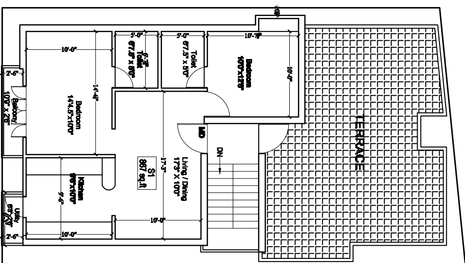
SECOND FLOOR PLAN(FINAL OPTION )
