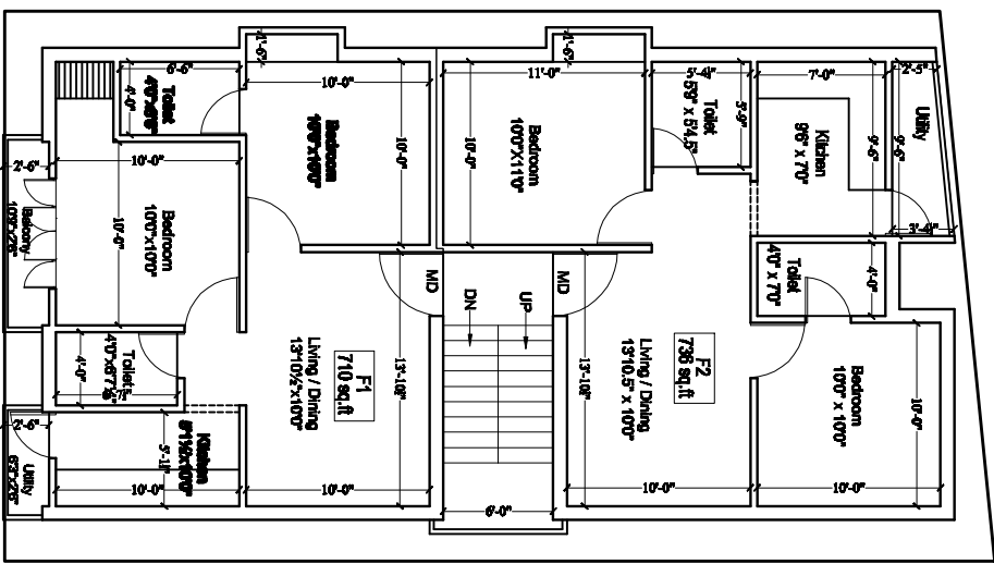
FIRST FLOOR PLAN (FINAL OPTION )
